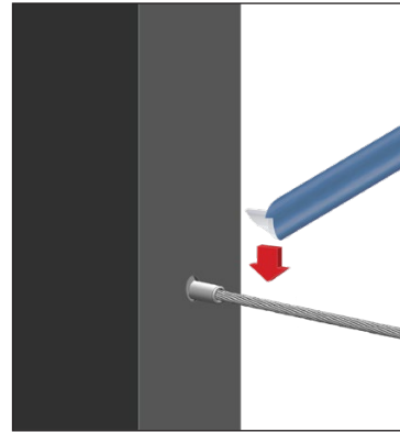
Figure BE. (LEFT) With the grommet install tool, push the cable grommet onto the cable in a downward motion.
