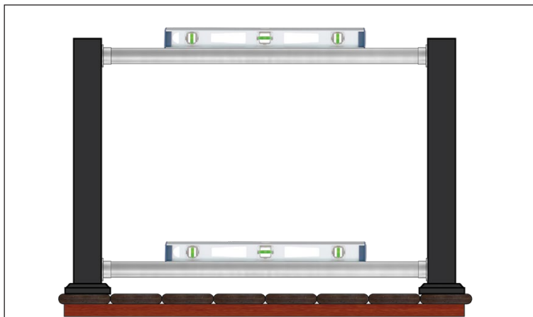
Figure H. With one sidemount installed, slide the other fitting against the opposite post. Slide it up or down until level
