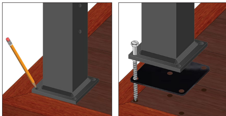
Figure C. (LEFT) When the final position is determined for the post, mark the hole locations of the four (4) 3/8" diameter mounting holes provided on the base and remove the post assembly.
