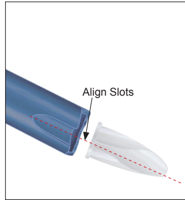
Figure BC (LEFT) Align the slot of the cable grommet with the slot of the tool. Figure BD. (RIGHT) Insert flange of cable grommet into the tool.
