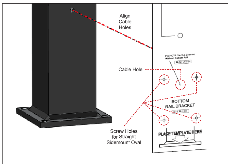
Figure B. Align the NOVA Nautilus drilling template against post and use a 5/32" drill bit to pre-drill your screw holes for straight sidemount oval. Pre-drill last cable hole using a 17/64" drill bit on post if installing top rail only.
